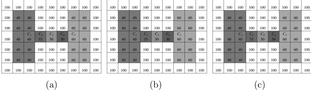
Fig. 1. (a) A schematic scene with each rectangular cell representing a single spel. A number in each spel indicates its intensity. We delineate an object indicated by a seed s = c_1 , assuming that its average intensity is m = 40 . We also assume \sigma = 1 . In (b) the shaded area depicts object P_{s,6}^\phi (i.e., with \theta = 6 ) delineated with the affinity \phi defined in (5). The region correctly excludes spel c_3 , since the difference between its intensity and m exceeds threshold value \theta = 6 . The shaded region in (c) represents object P_{s,6}^\kappa , where \kappa(c, d) = \left| \frac{f(c)+f(d)}{2} - m \right| . Not only it incorrectly leaks all the way to spel c_5 , but it also abruptly stops there, after reaching an area of uniform intensity.
