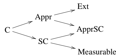
Chart 5. Approximately and symmetrically continuous functions.
