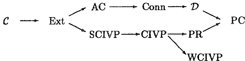
Chart 2: "Darboux like" functions.
