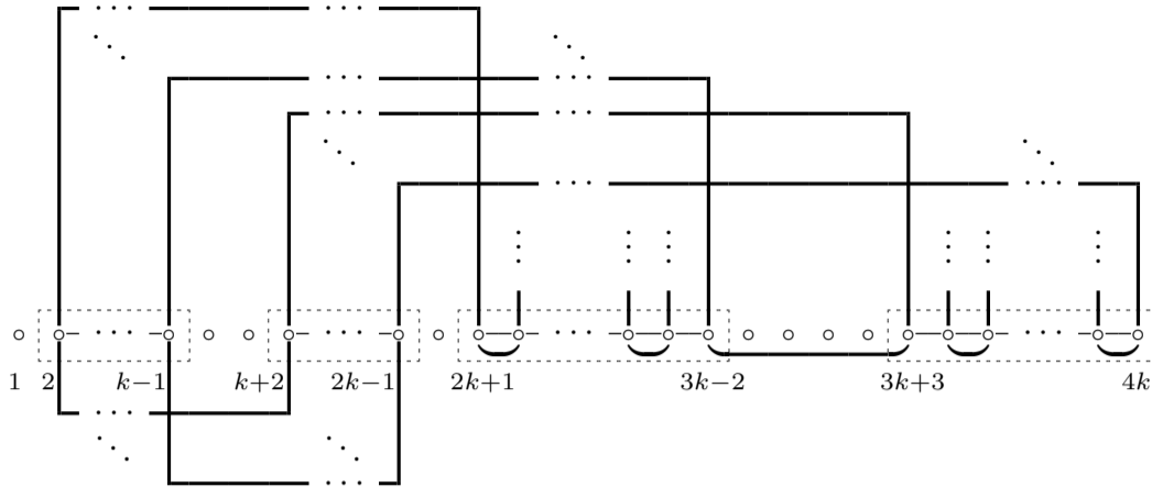
Fig. 3. The graph G_3 .
