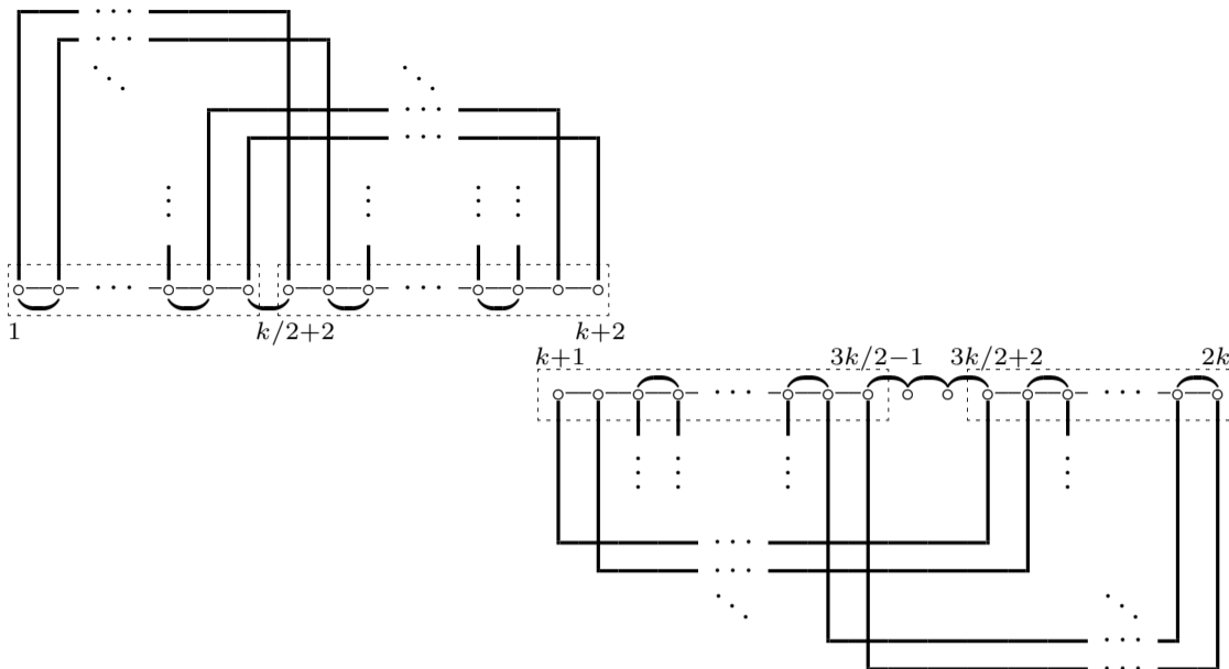
Fig. 8. The cycle C^{(2)} .
