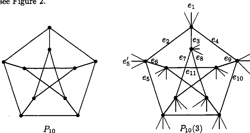
Figure 2 The Petersen graph P_{10} and P_{10}(3)
