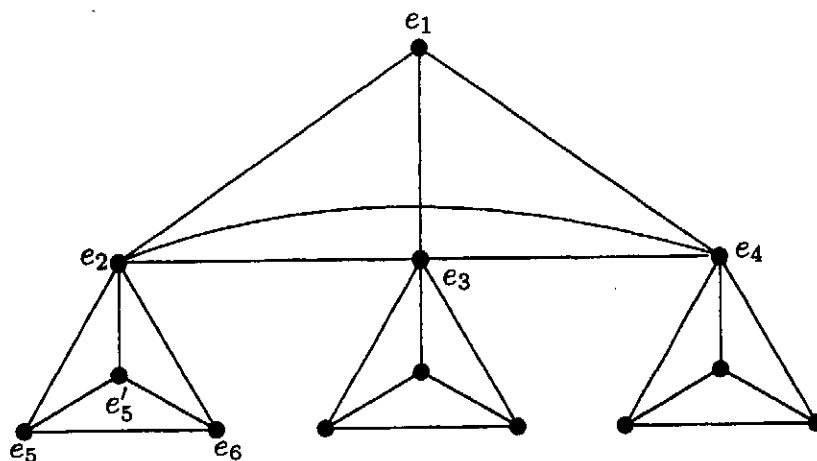
Figure 3 An illustration of the proof that e_1 is locally N^2 -connected in G(k)
