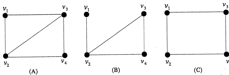
Fig. 1. Examples of perfect b -matchings
