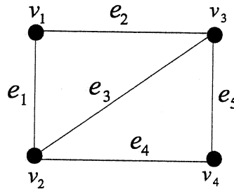
Fig. 3. Examples of T -joins
