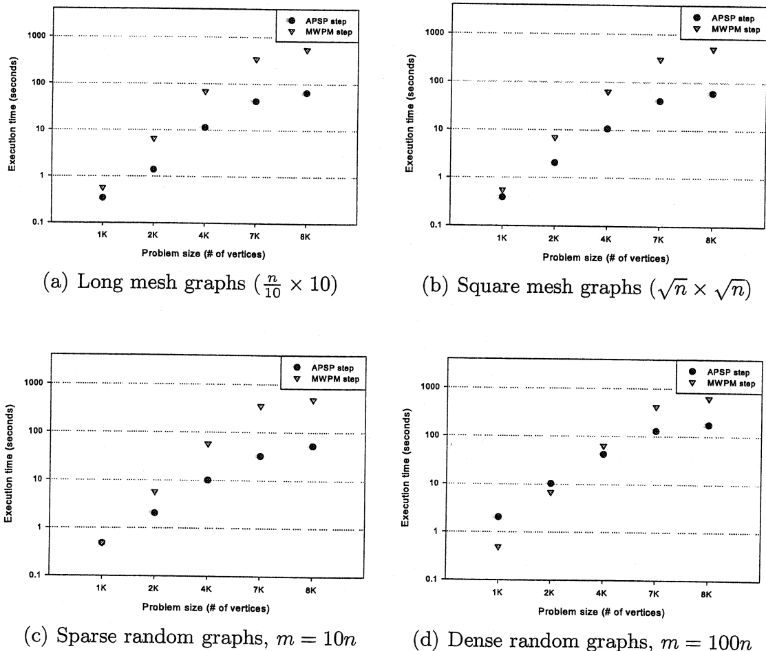
Fig. 4. Execution time of the APSP and MWPM steps for various graph instances
