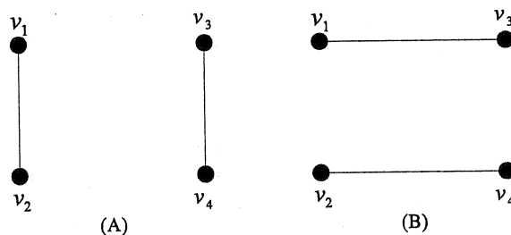
Fig. 2. Examples of perfect matchings
