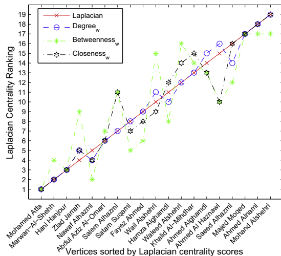
Fig. 5. Ranking information based on all centrality methods for these 3 data sets considered here. (Top) The 32 scientists in Freeman's EIES network; (Middle) 34 actors in Zachary's karate club; (Below) these 19 hijackers in the 9/11 hijacker network.
