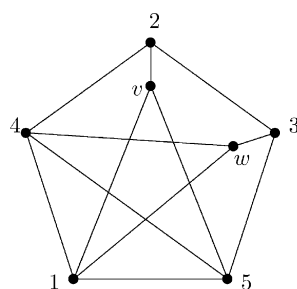
Fig. 14. A (P_{10})_{\bar{3}} -minor.
